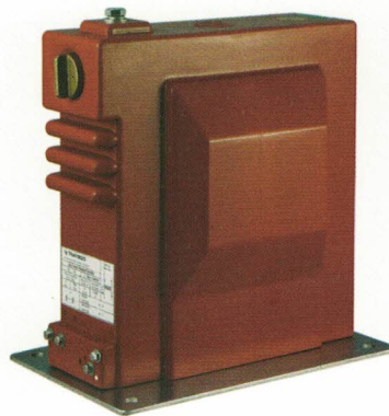
VT-24F
